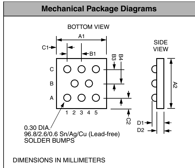
Package Dimensions for CSPEMI205 Chip Scale Package
