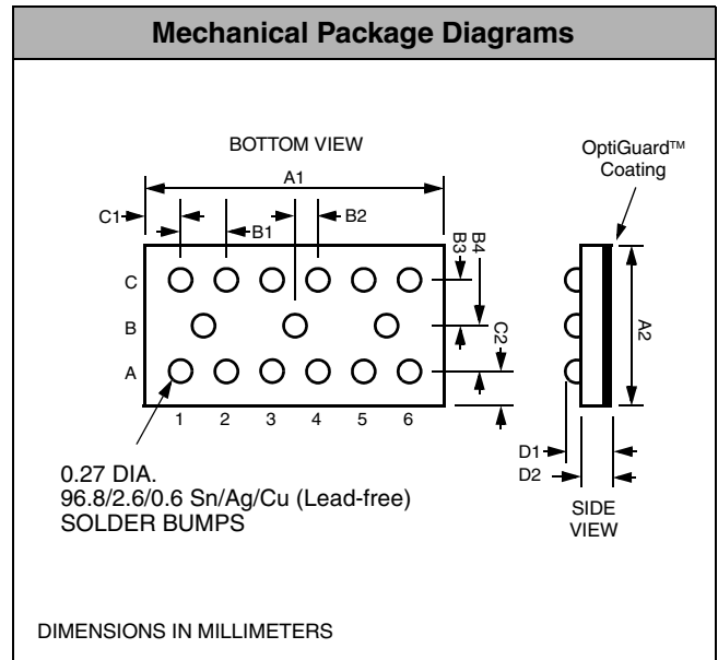
Package Dimensions for CM1453-06CP Chip Scale Package
