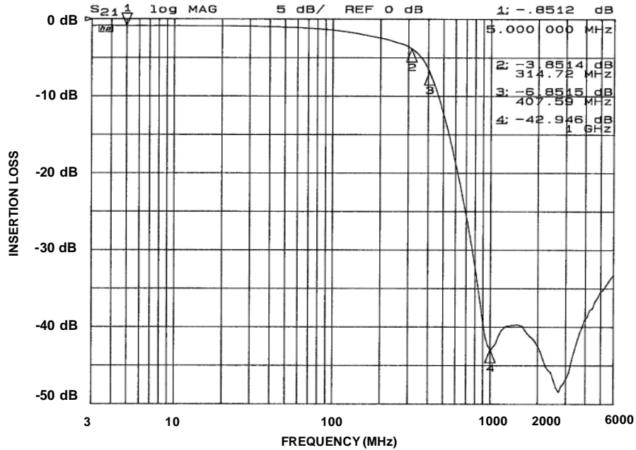
Figure 1. Insertion Loss VS. Frequency (CM1453-06: Filter 1)
