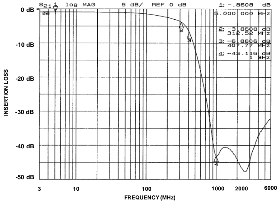
Figure 4. Insertion Loss VS. Frequency (CM1453-06: Filter 4)
