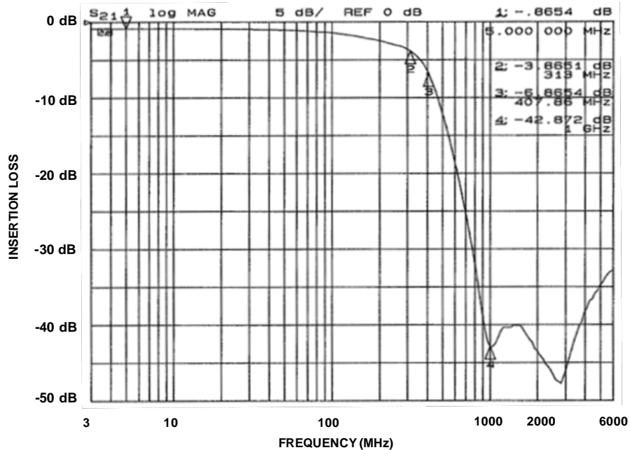
Figure 2. Insertion Loss VS. Frequency (CM1453-06: Filter 2)
