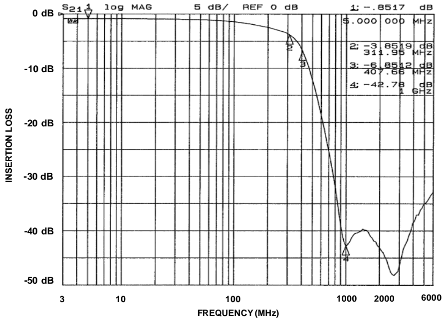
Figure 5. Insertion Loss VS. Frequency (CM1453-06: CSP1 – Filter 5)
