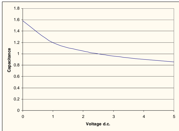
Figure 7. Typical Diode Capacitance vs. Input Voltage (normalized to 2.5V d.c)
