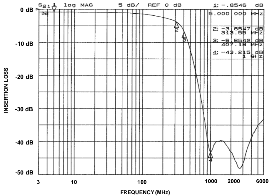
Figure 6. Insertion Loss VS. Frequency (CM1453-06: CSP1 – Filter 6)
