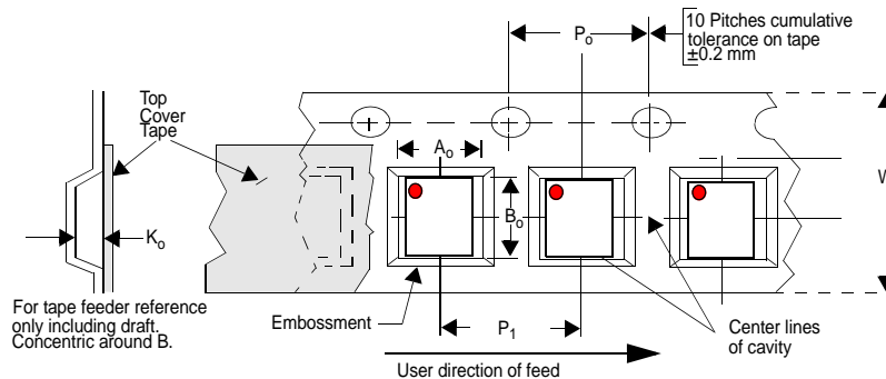
Figure 6. Tape and Reel Mechanical Data
