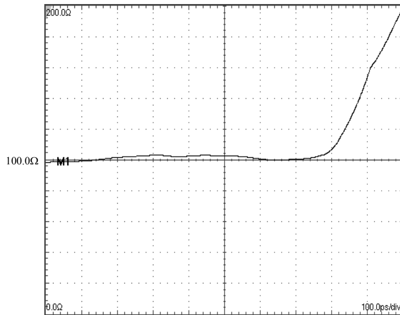
Figure 7. Typical Channel TDR Measured Across Out_x and In_x Per Each Differential Channels Pair (Typical 200ps Incident Rise Time)
