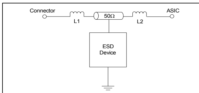
Figure 3. CM1236 PicoGuard XS ESD Protection Model
