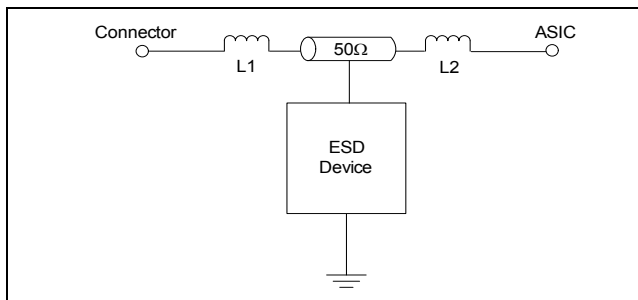
Figure 3. CM1235 PicoGuard XS ESD Protection Model
